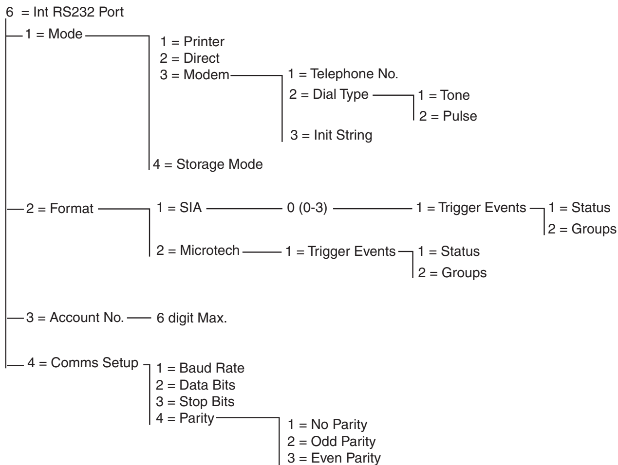
Figure 9. Internal RS232 Programming structure
