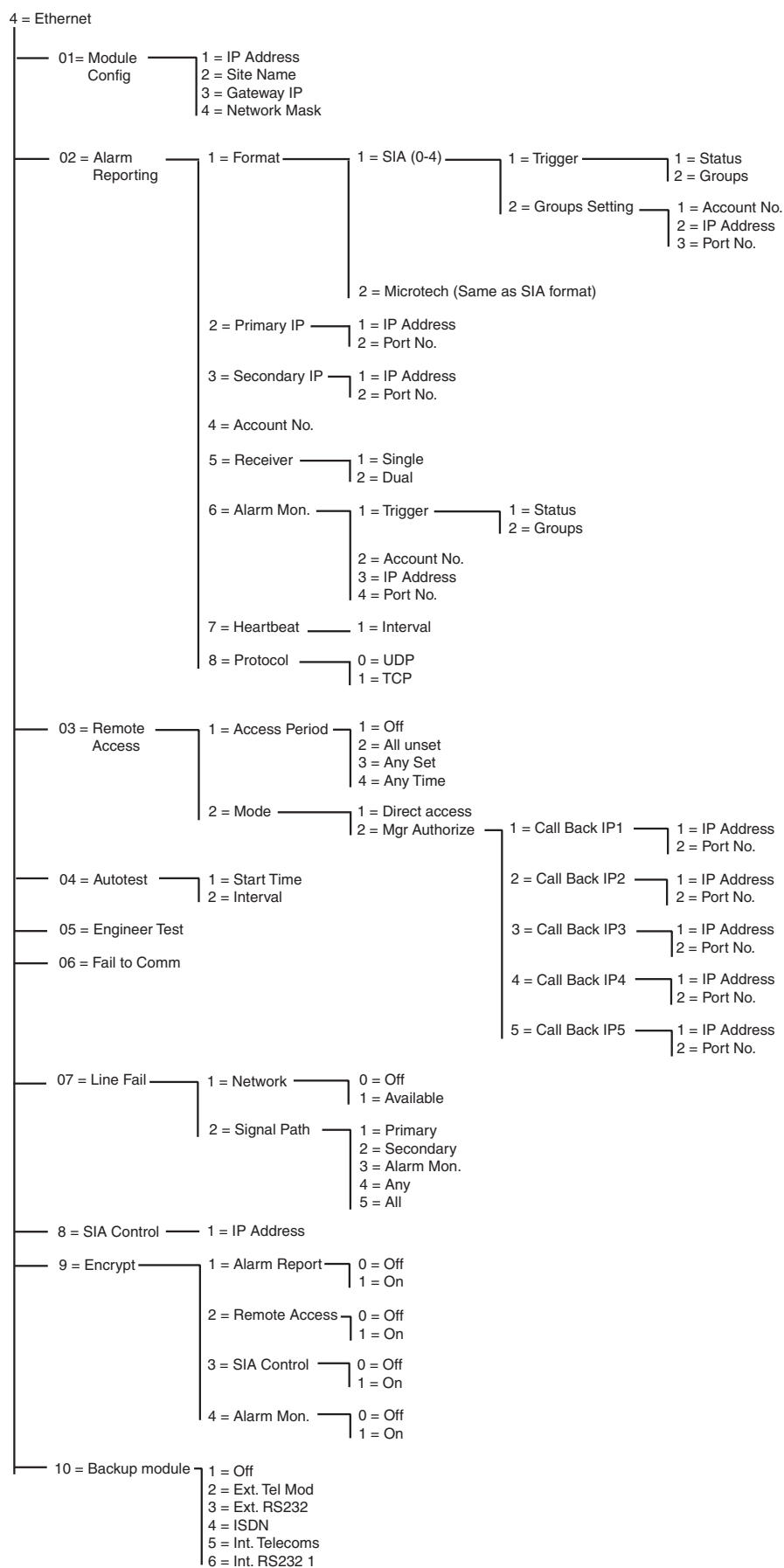
Figure 8. Ethernet Module Programming Structure
