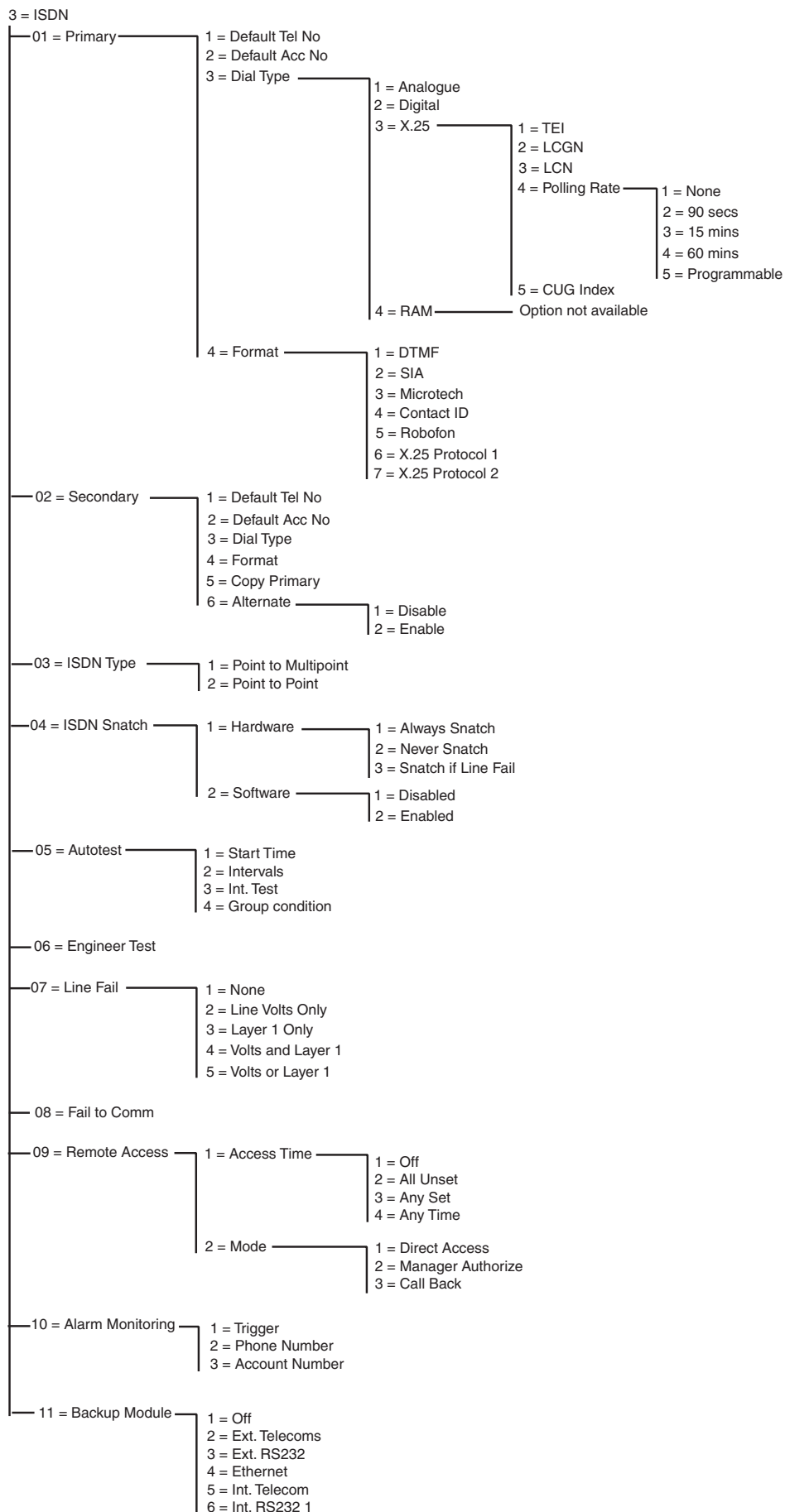
Figure 7. ISDN Programming Structure
