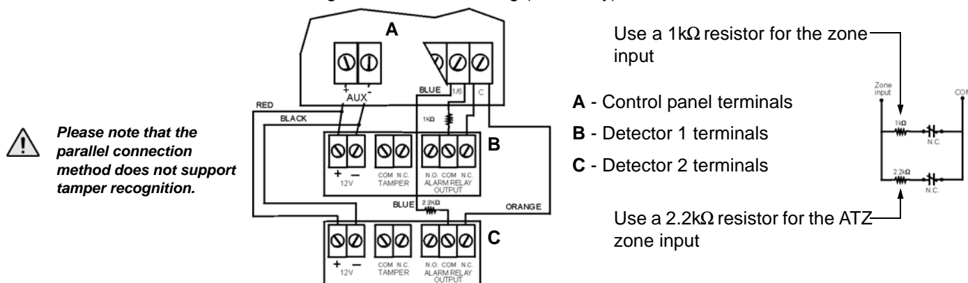
Figure 17: Parallel Wiring (1728 only)
