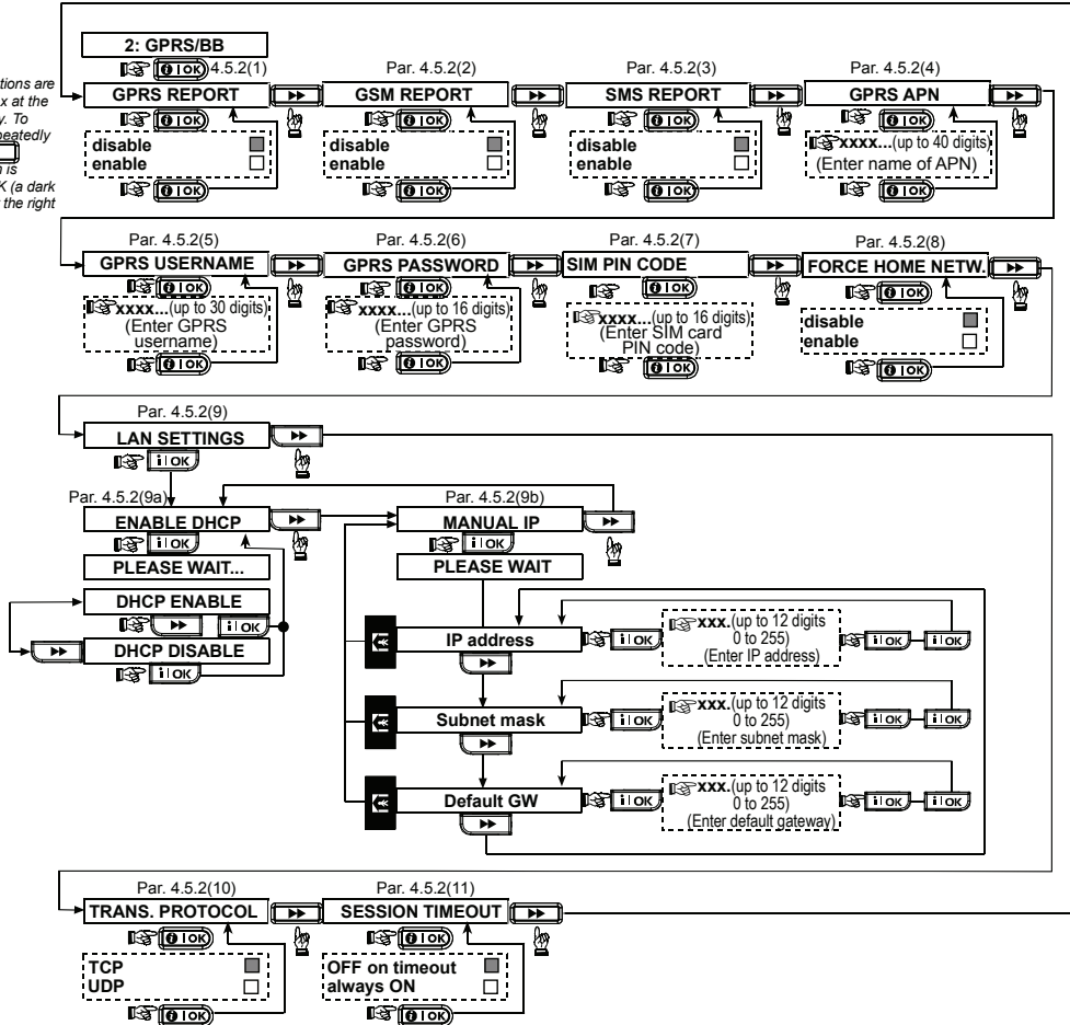
FIGURE 4.5 - DETAIL B
