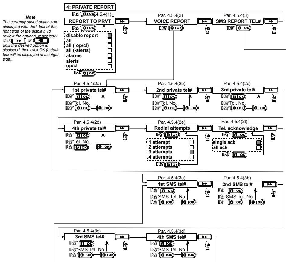
FIGURE 4.5 - DETAIL D
