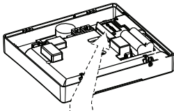
Figure 3.4 - Optional GSM Module Mounting
