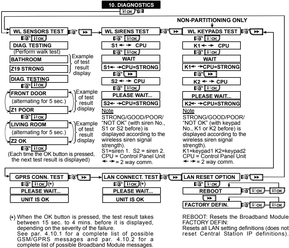
Figure 4.10 - Diagnostic Test Flow Chart
