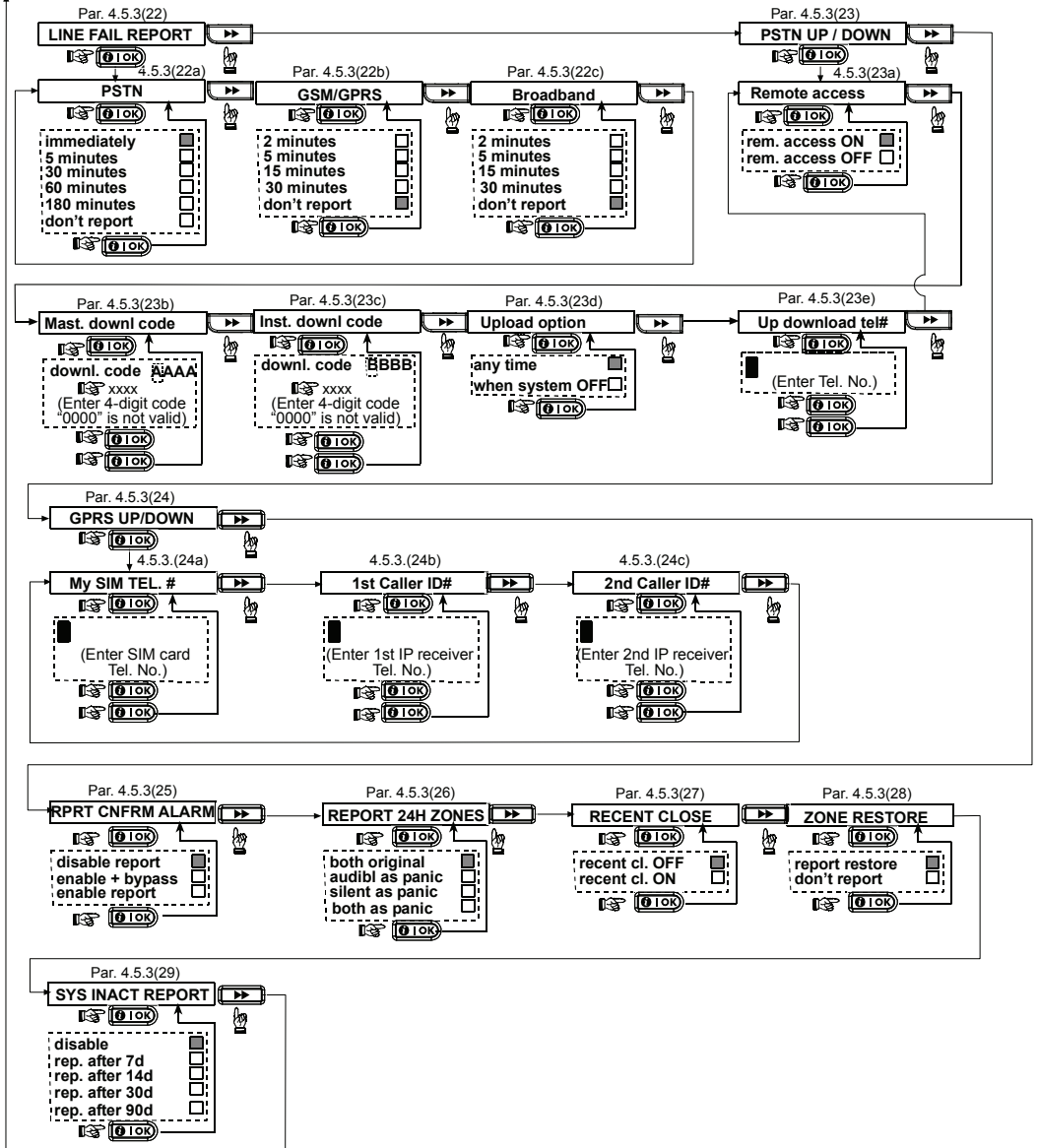
FIGURE 4.5 - DETAIL C continued
