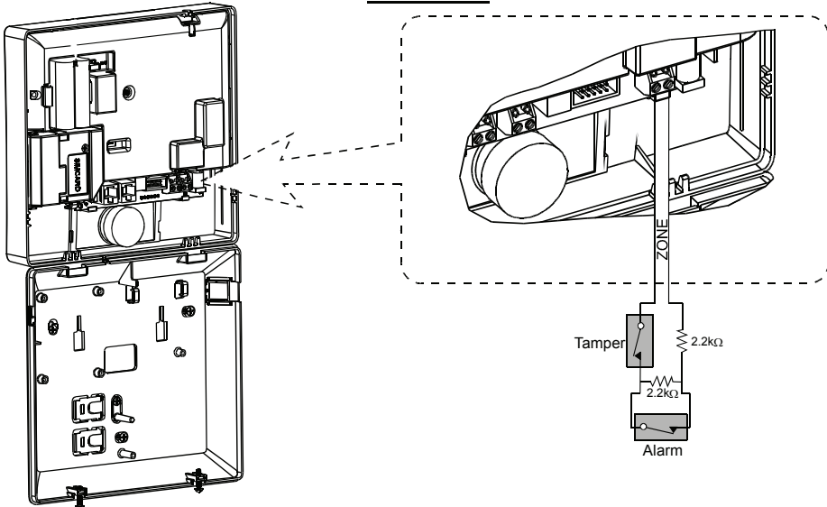
Figure 3.2 - Wiring
