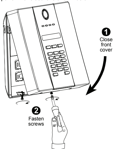
Figure 3.7 - Final Closure
