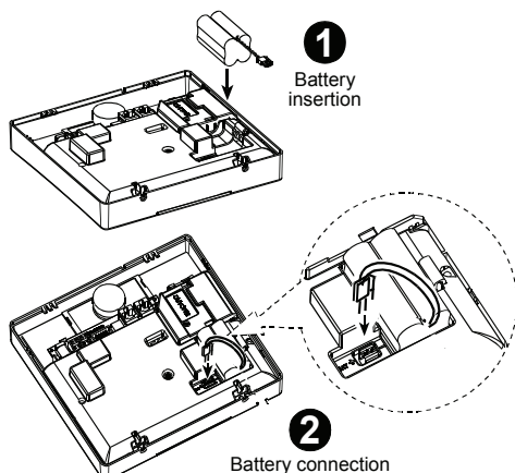
Figure 3.3 - Battery Insertion
