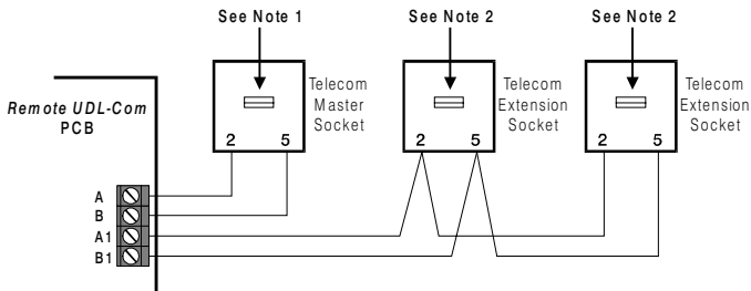
Figure 3. PSTN Connections
