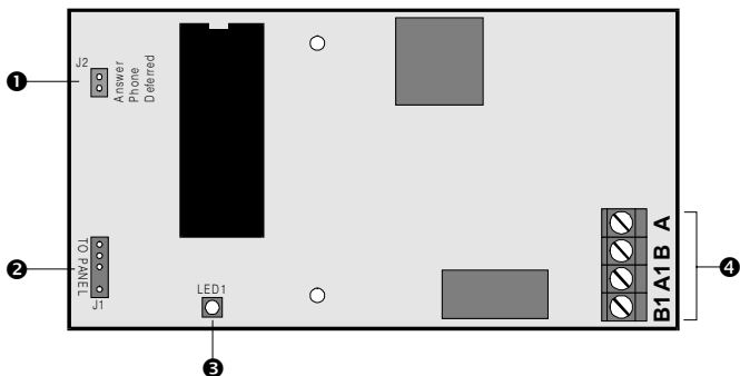
Figure 1. UDL-Modem PCB Layout
