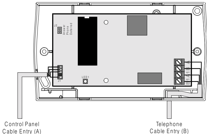
Figure 2. Cable Routing
