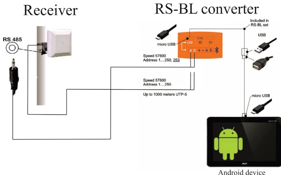
Fig.10.2 FMC 24 CONNECTION WITH RS-BL AND ANDROID DEVICE VIA WIRES
