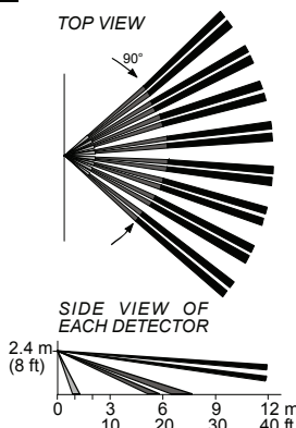
Fig. 2 - Coverage pattern
