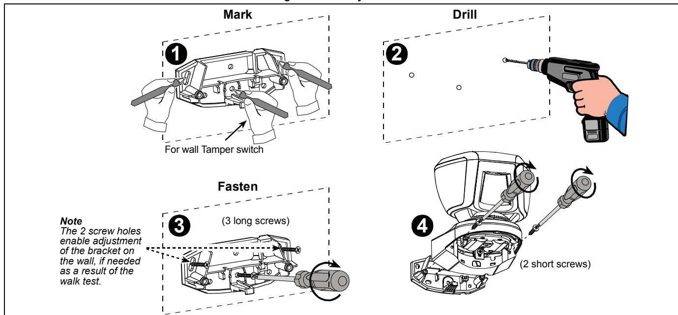
Figure 4 - Installation
