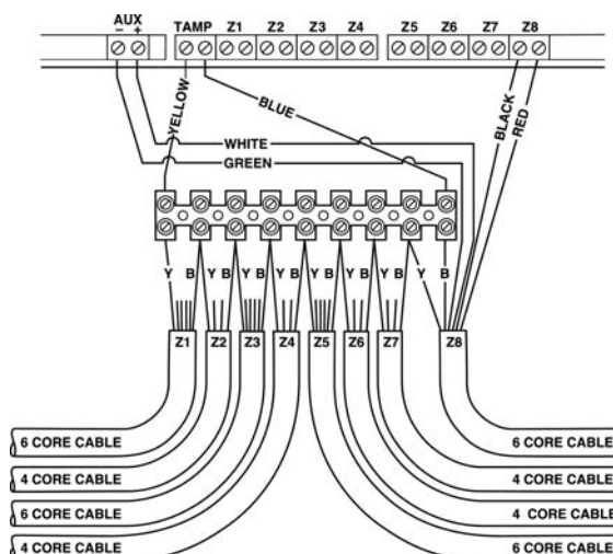
Figure 6 - Wiring the Global System Tamper
