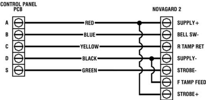
Figure 3e - Gardiner Technology Novagard 2
