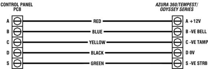
Figure 3a - Texecom Azura 360/ Tempest/Odyssey Series
