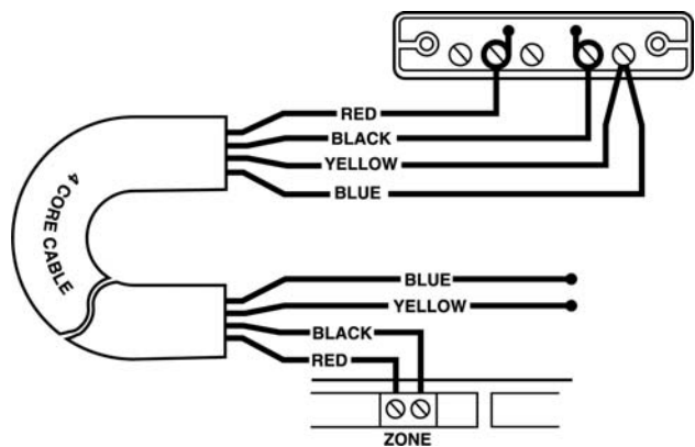
Figure 4 - Wiring Magnetic Contacts
