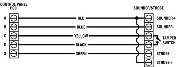
Figure 2 - Typical SAB Connections
