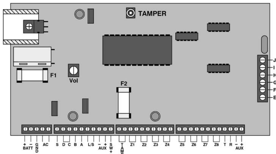
Figure 1 - Control Panel PCB Layout
