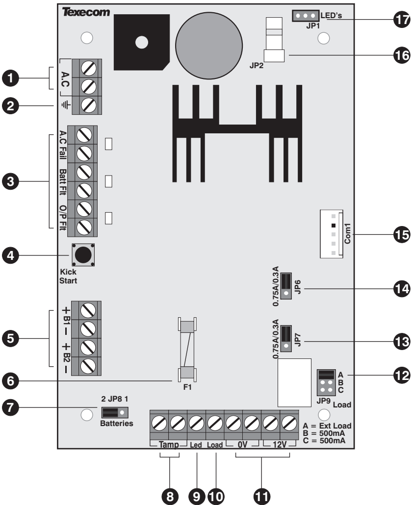
Figure 2. PCB Layout
